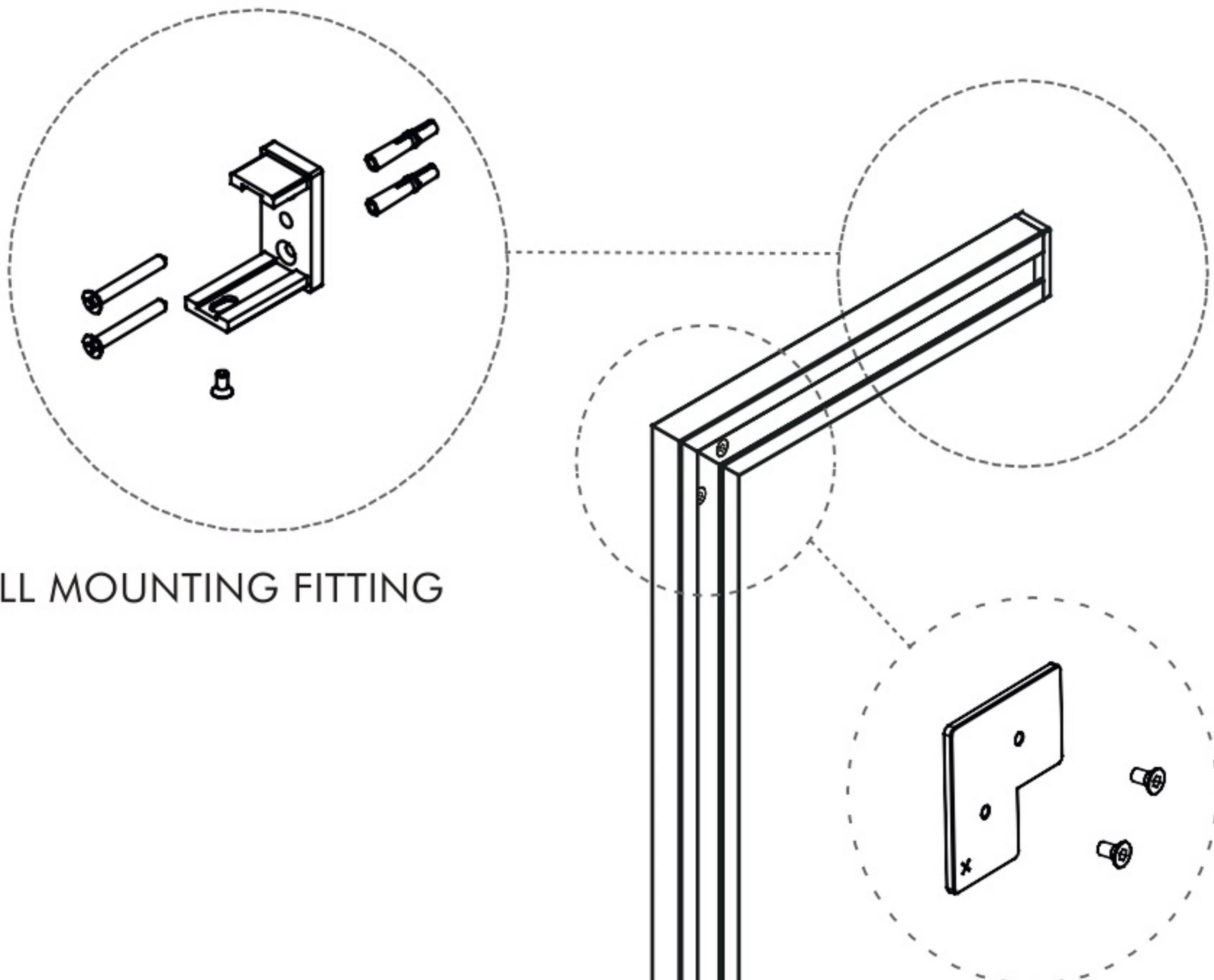
CORNER CONNECTOR
